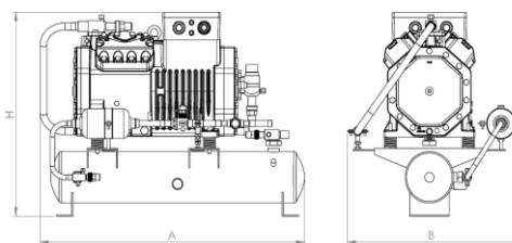
4TES-9Y/RHC15B - 6FE-50Y/RHC60B
